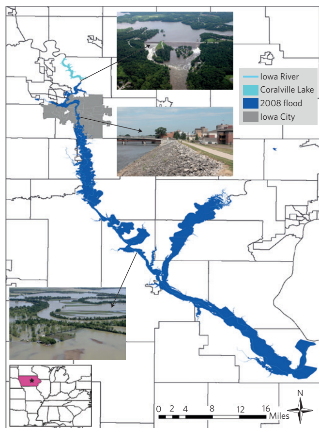
Figure 2 | Iowa River study area near Iowa City, Iowa, USA. This map shows Coralville Dam with flooding spillways and the extent of the 2008 flood that breached some levees in Iowa City (urban footprint shown in grey) and extensively inundated downstream floodplain farmland and riparian habitats (dark blue).
